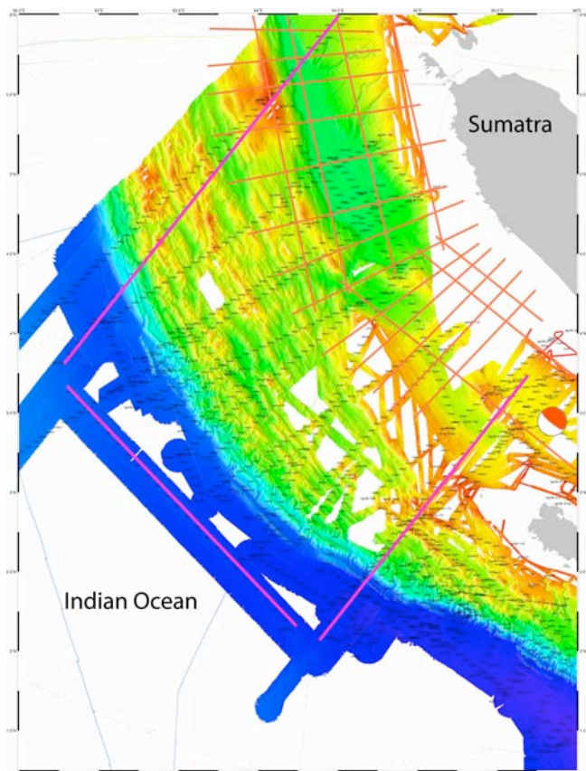
Figure: The 2004 great Andaman Sumatra earthquake epicentral region (Red beach ball). Black lines are US seismic profiles, Red lines: TGS seismic profiles, and Purple lines: Schlumberger deep seismic profiles.
